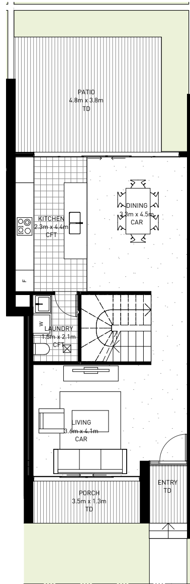
GROUND
